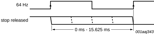
Fig 25. STOP bit release timing
