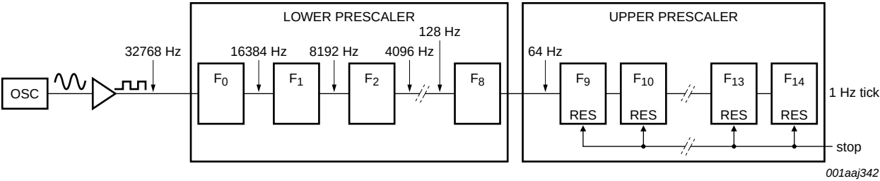
Fig 24. STOP bit functional diagram
